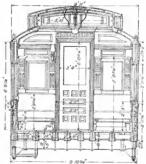
Fig. 445. Transverse Section.
